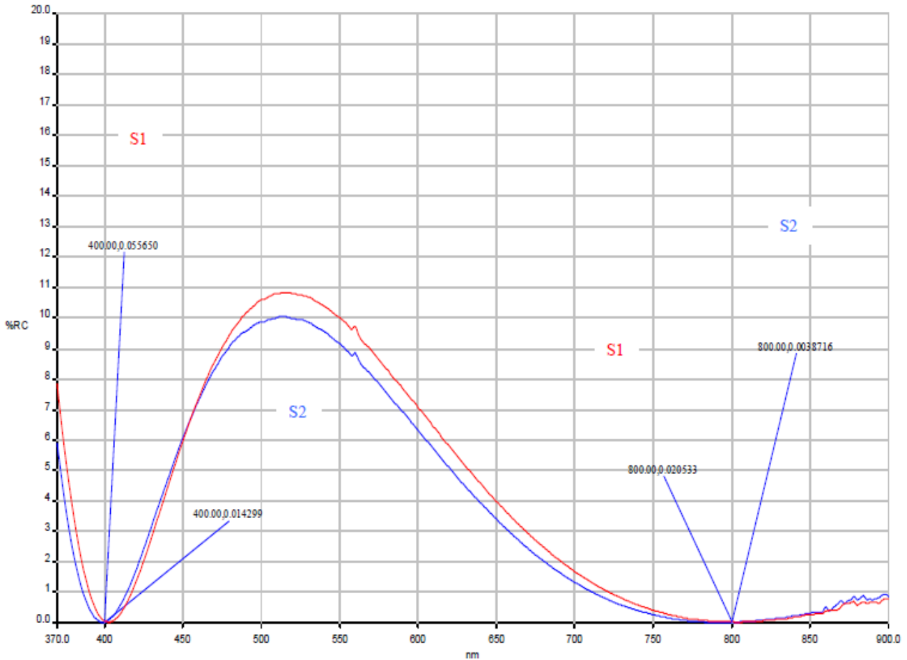
Reflection curve
